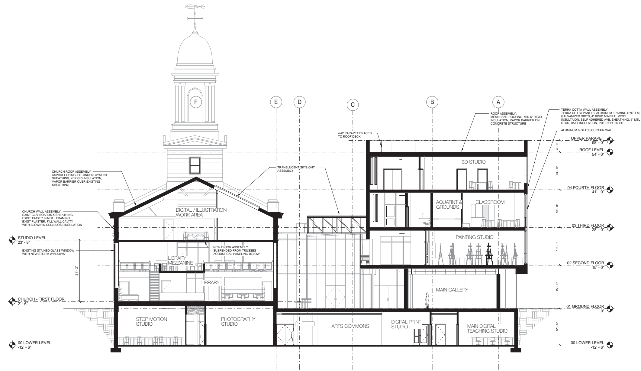
Gallery + Library Cross Section Looking West 1" = 20'-0"
